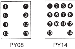
Terminal Arrangement (Bottom View)
